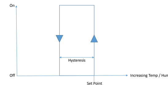
Rising Control with positively (+) biased set point
