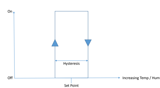
Falling Control with negatively (-) biased set point
