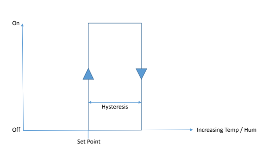
Falling Control with positively (+) biased set point
