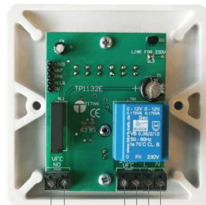
Volt free output Max 240V 5amp Supply 24V AC/DC - TPEXT1/24 240V AC - TPEXT1/240 Remote start Fit link for normal operation
